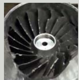
Impeller damage
